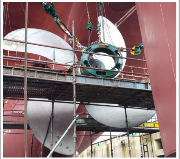
PROPELLER INSTALLATION
