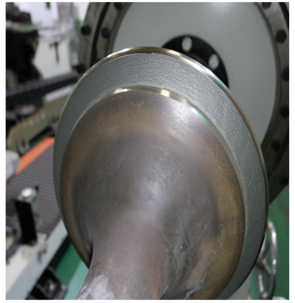
CLADDING OF EX.VALVE SPINDLE LID SURFACE
