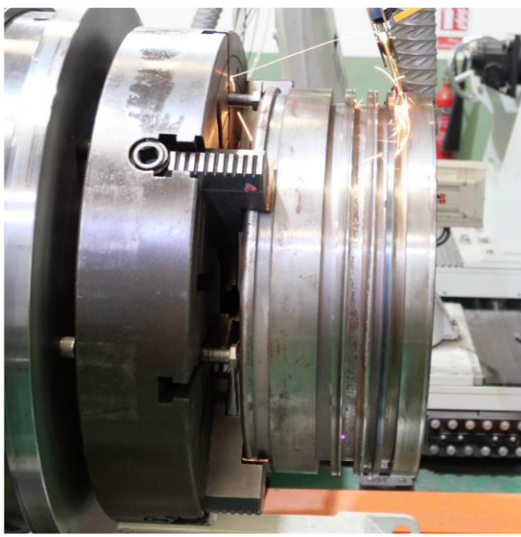
CLADDING OF PISTON RING GROOVES
